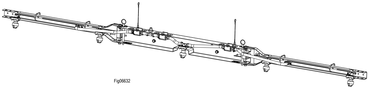
Boom Assembly
